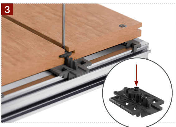
Fit all boards and tighten screw
