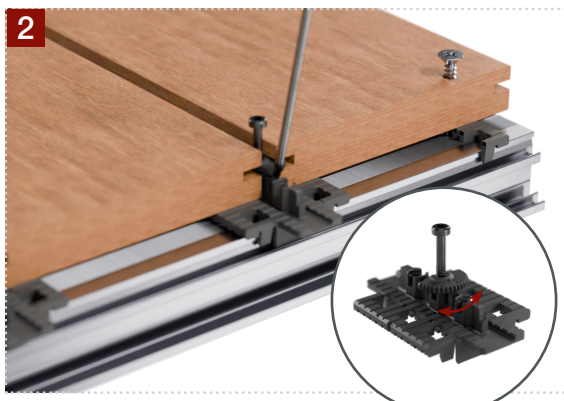
Rotate Fastening Disc
