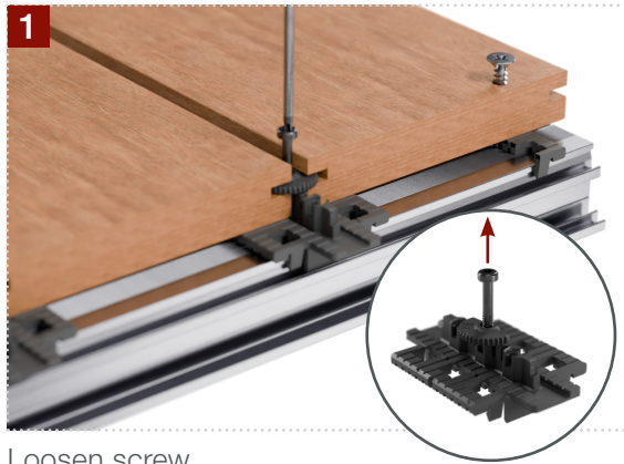
Loosen screw
