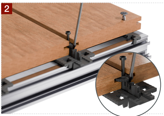
Fit board and rotate Fastening Disc
